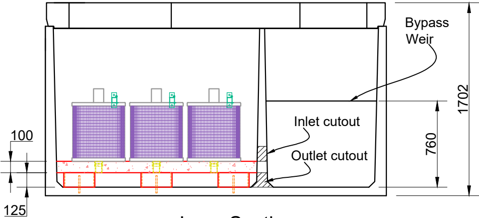
Long Section
